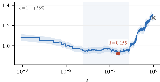
Falcon3-7B, \rho=40\% (339 solutions)
