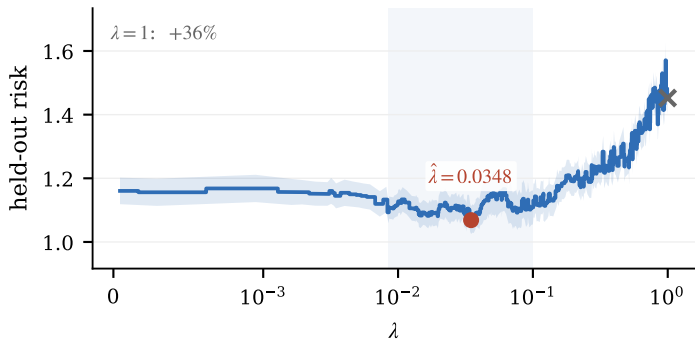
Llama-3.1-8B-It, \rho=30\% (350 solutions)
