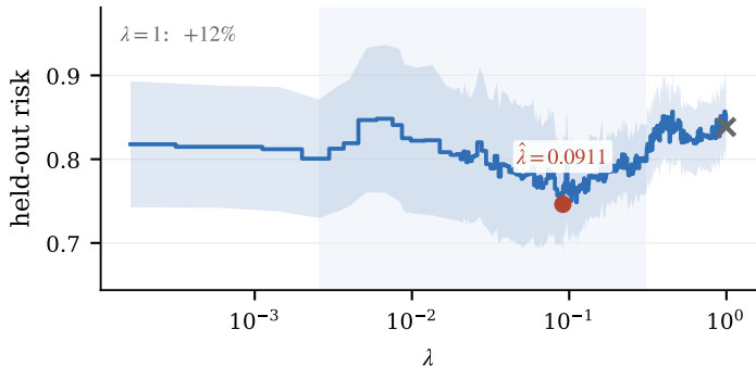
Llama-3.2-3B, \rho=20\% (288 solutions)
